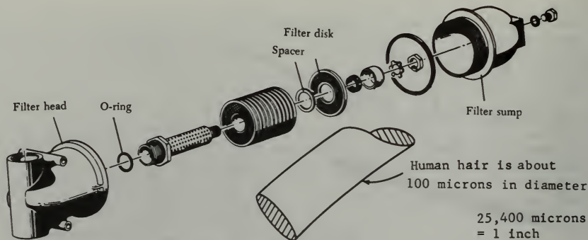
FIGURE 3-57. Wafer screen filter.
